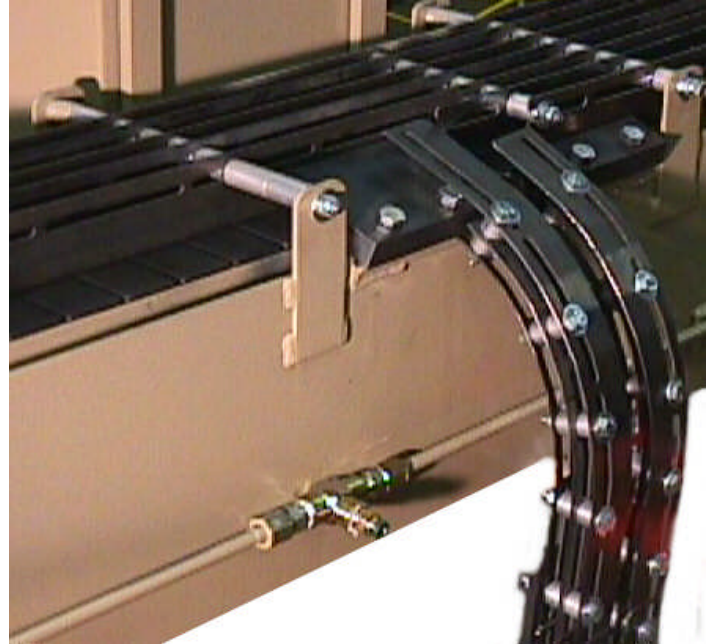
Waterfall From Distribution Conveyor Shown
