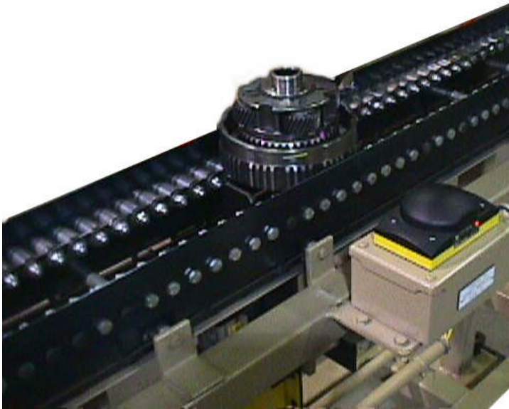
Straight Split Gravity Roller with Back-Up Rail Shown
